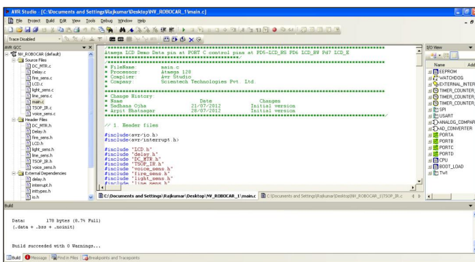
Program Window
