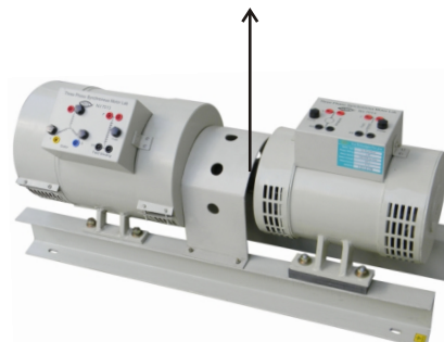
AC Motors -Generator Set Coupled with Flexible Lovejoy Coupling
