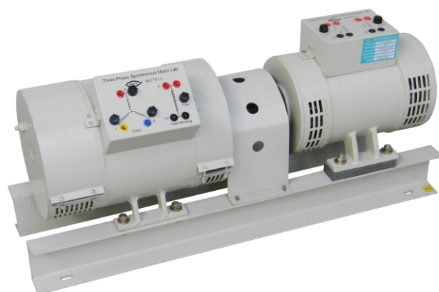
Generator with Electrical loading arrangement
